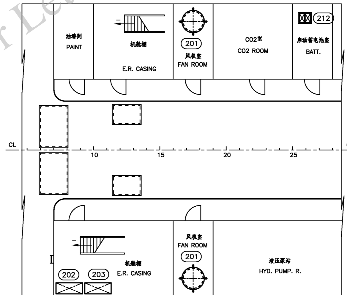
拖网甲板 TRAWL DECK
